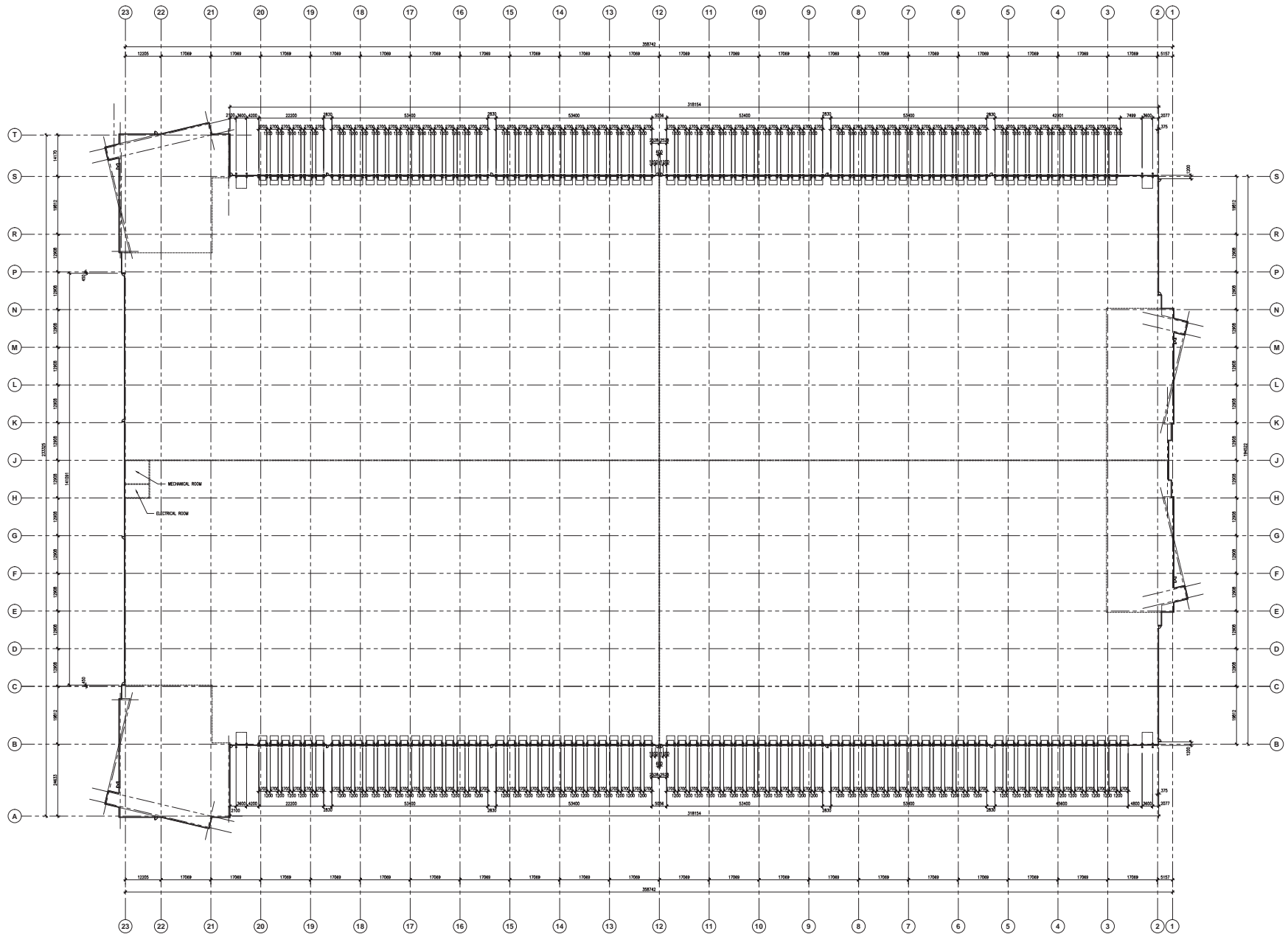
1. GROUND FLOOR PLAN
